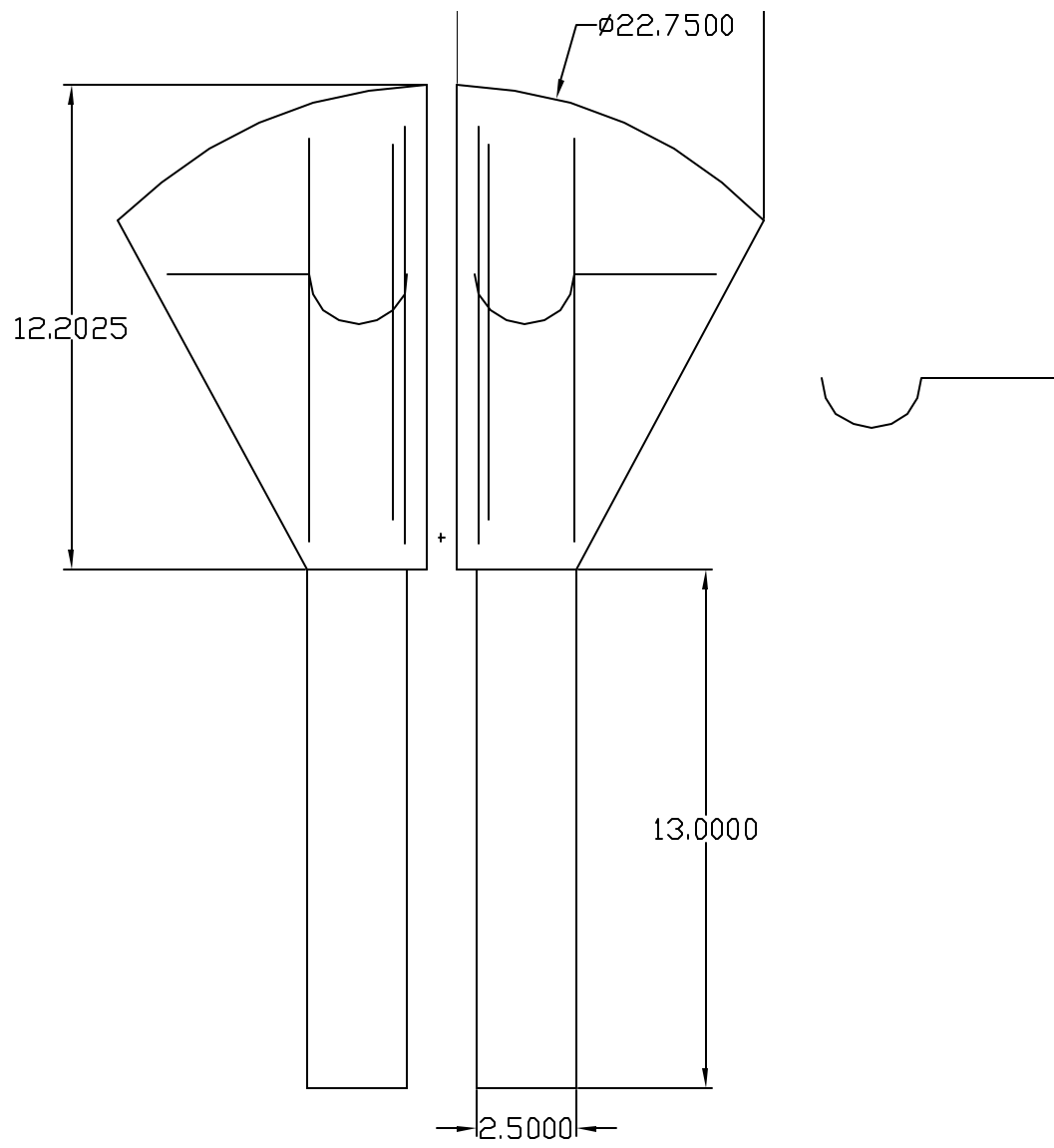
Burner Tube and lift plate
