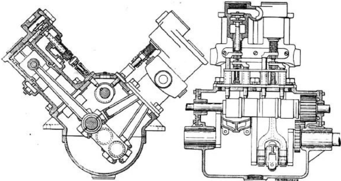
FIG. 1. THE NEW DIETER STEAM ENGINE.
