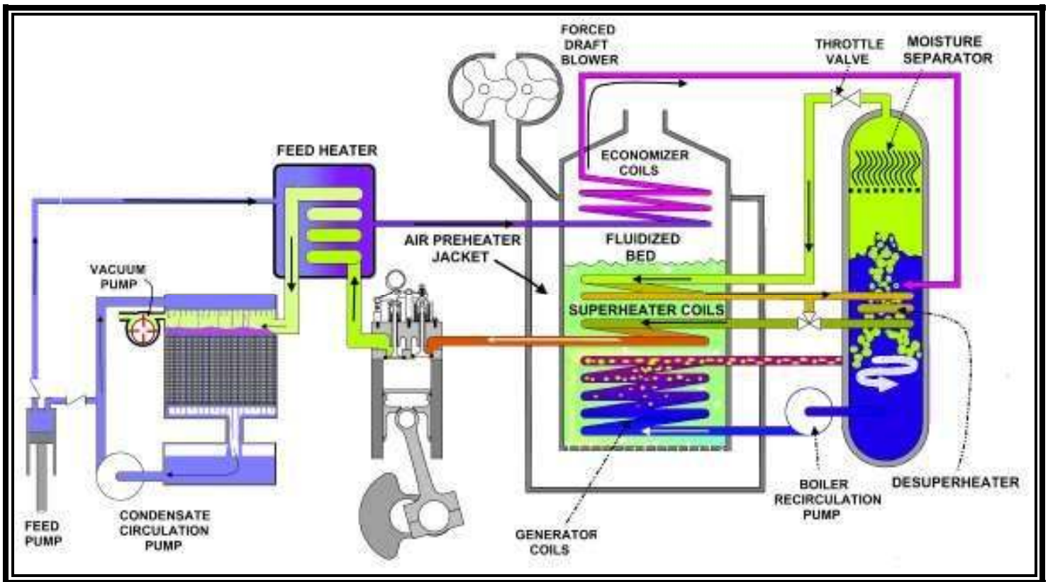
SIMPLE STEAM SYSTEM SCHEMATIC
